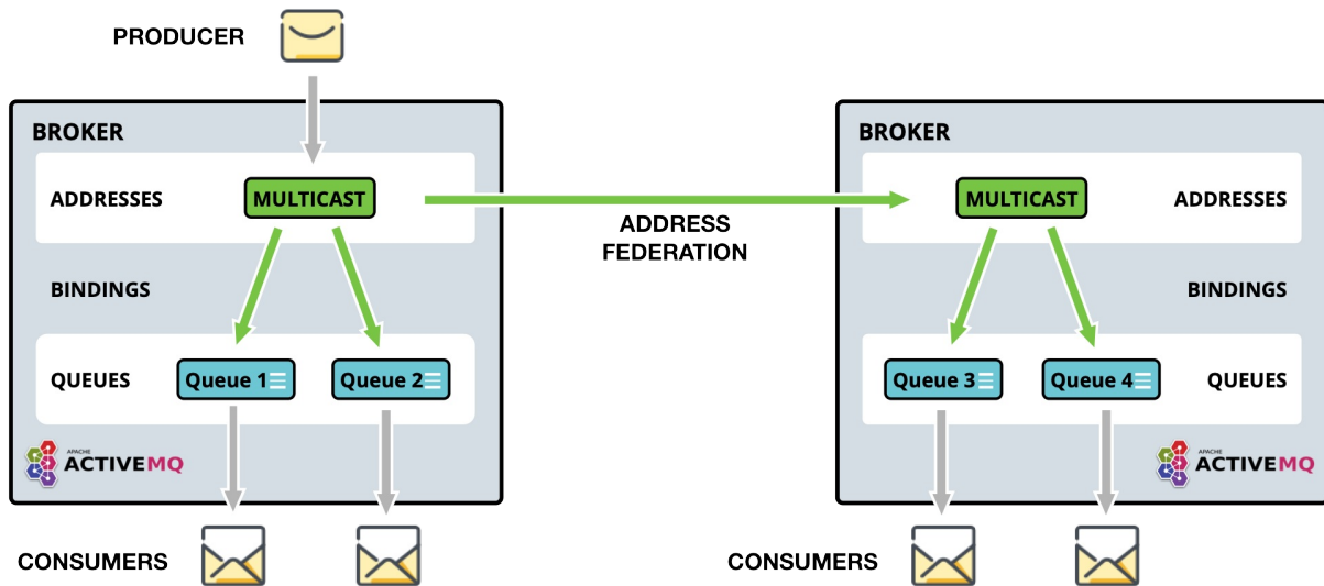
Figure 1. Address Federation
