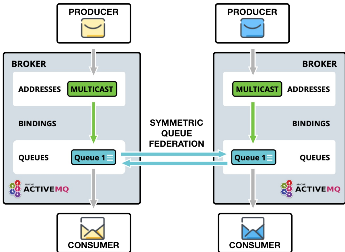
Figure 2. Queue Federation
